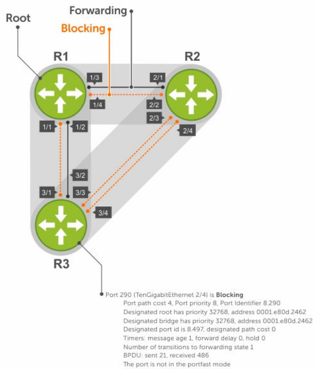
Figure 112. Spanning Tree Enabled Globally
